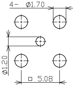
RMD PCB Mounting Hole
