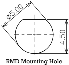
RMD Mounting Hole
